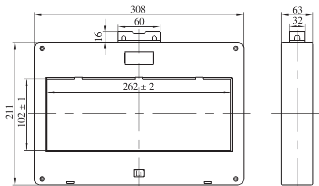
BT3/6300 for three poles
