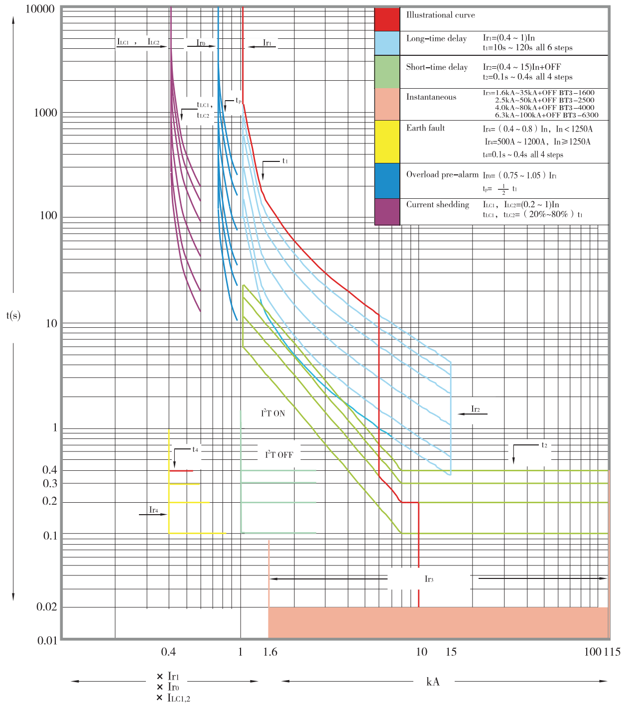
T/I (time / current) curve of uncommon inverse time It of type EA, EP and EQ intelligent controllers
