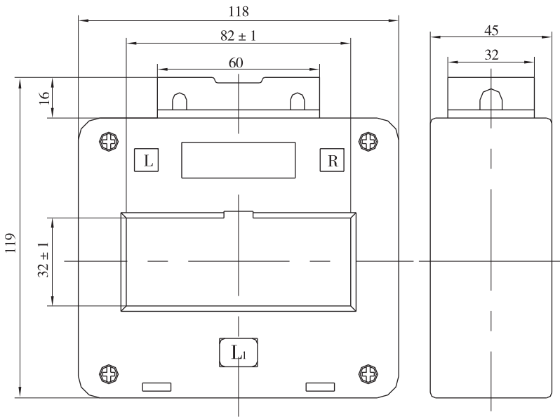
BT3-2500 for three poles
