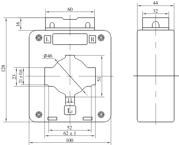
BT3-1600 for three poles
