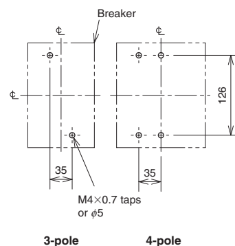
Drilling plan
