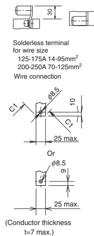
Conductor drilling for direct connection
