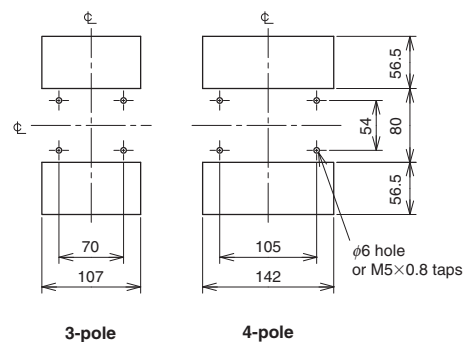
Drilling plan
