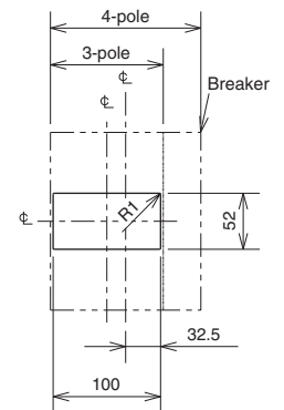
1mm clearance on each side of the handle frame
