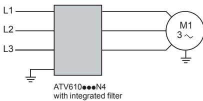
Altivar Easy 610 drive with integrated EMC filter
